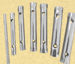
AUTOGEAR SPANNER TUBE SET 7 Piece set 8-19mm
