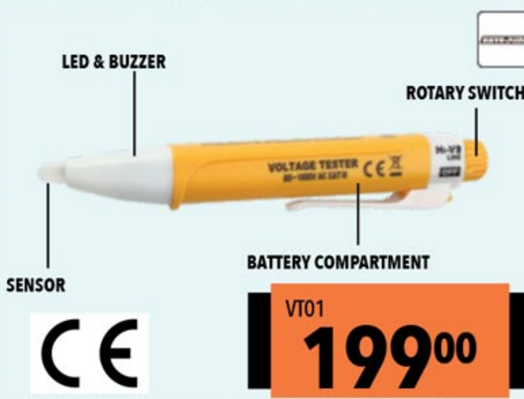
AUTOGEAR ADJUSTABLE NON-CONTACT VOLTAGE TESTER
